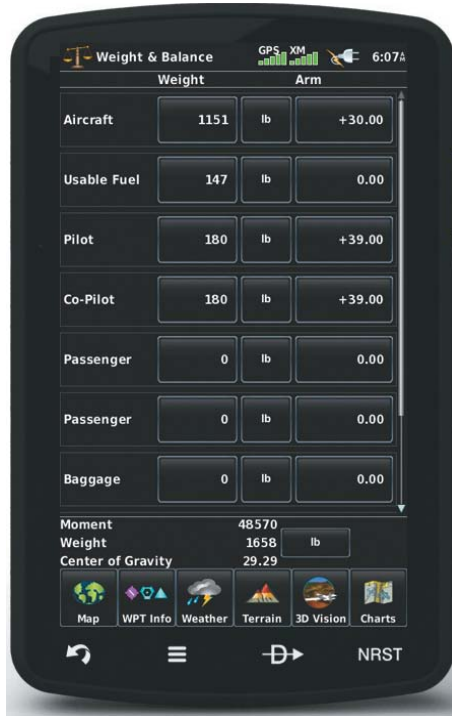
Weight & Balance
