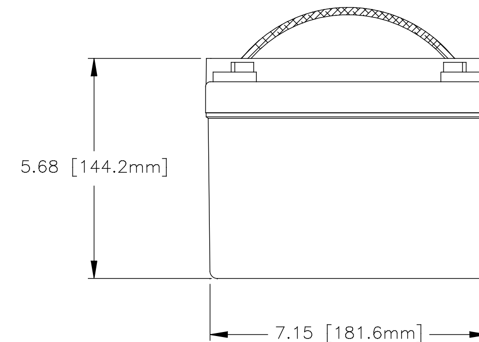
ENVELOPE DRAWING
